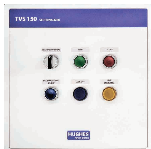
Front panel
